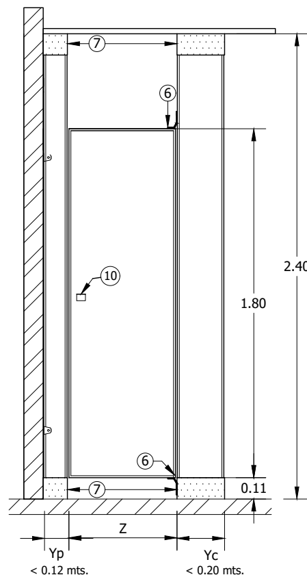
VISTA FRONTAL
